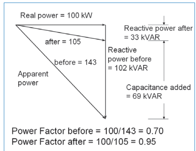
Figure 4. Effect of Power Factor Correction
