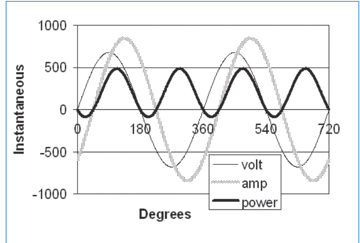
Figure 2. 0.7 Power Factor at 200kW
