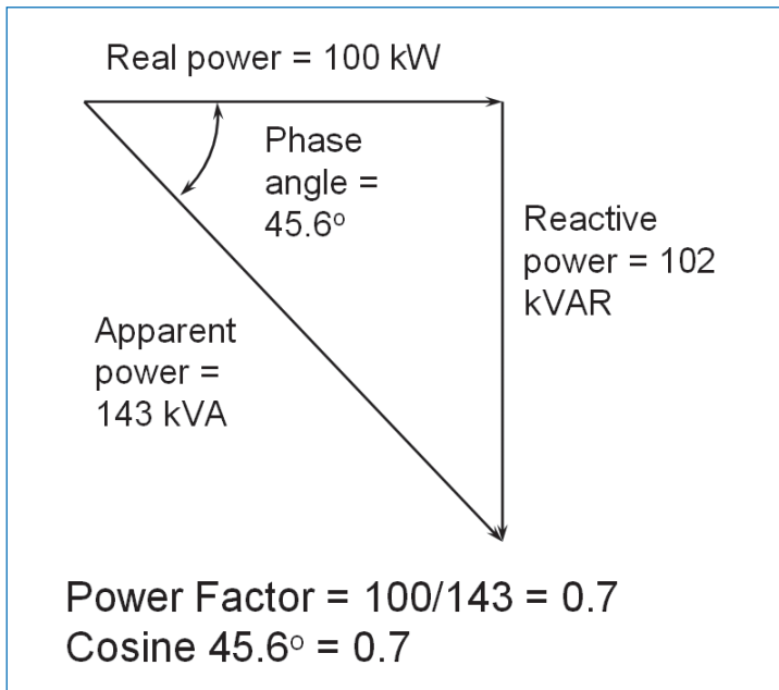
Figure 1. Power Triangle
